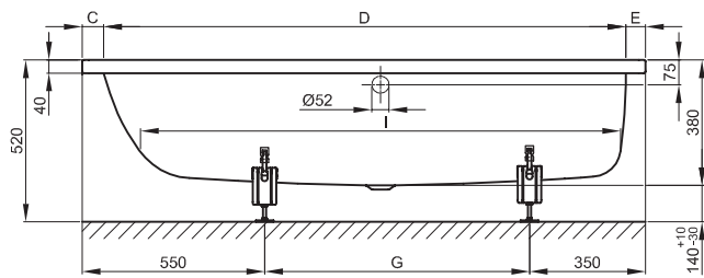
foot end right and overflow rear, article no. 8836
