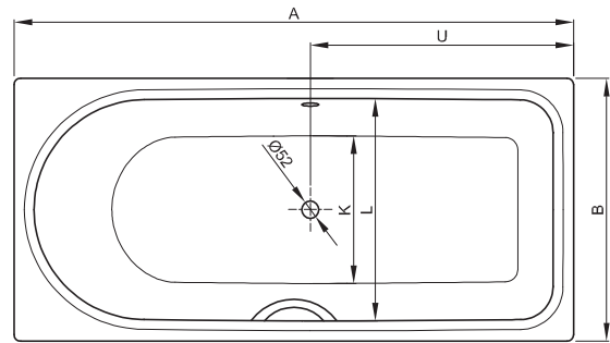
foot end right and overflow rear, article no. 8836
