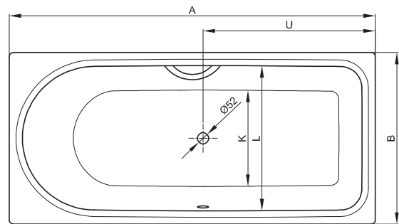
foot end right, overflow front, article no. 8837
